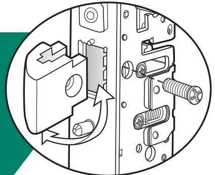
Field Reversible Latch Bolt
